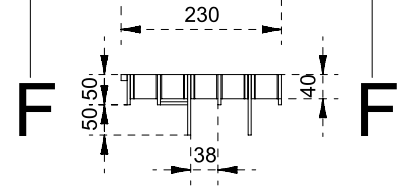
SECTION F-F
