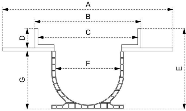
GRATE, FRAME AND PREFORMED TRENCH
